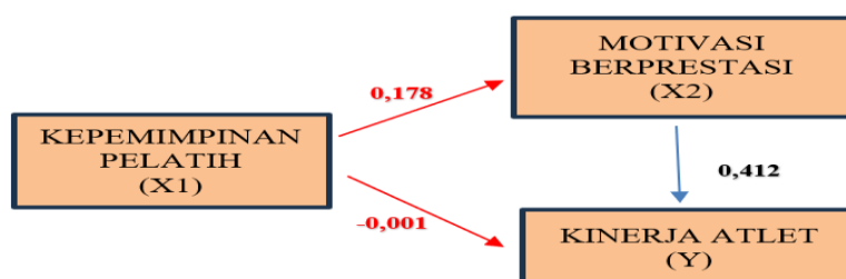
Figure 6. Final Path Analysis Model
